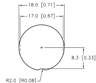
MOUNTING HOLE
